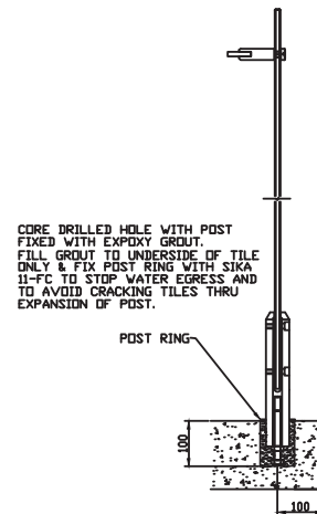
CORE DRILL FIXING
