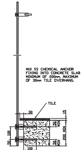
SIDE FIX CONCRETE SLAB
