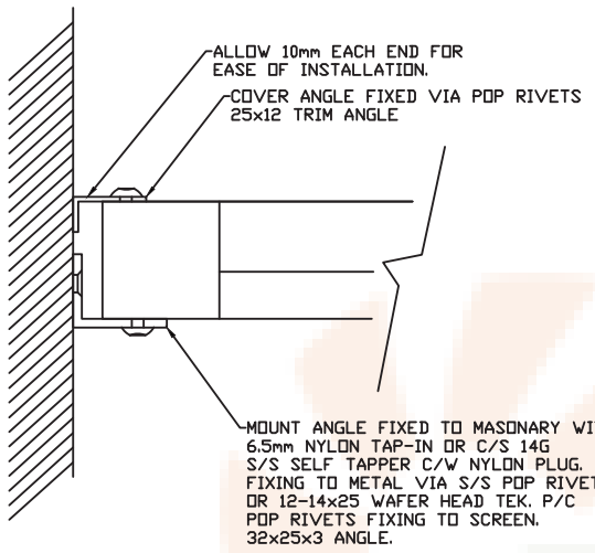
FIXING DETAIL
